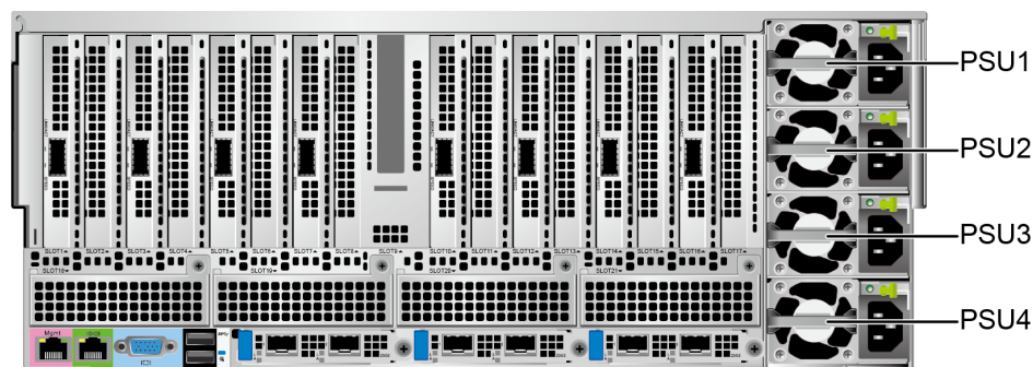
Figure 5-40 Power module location (example: 24 x 3.5" Drive Configuration))
