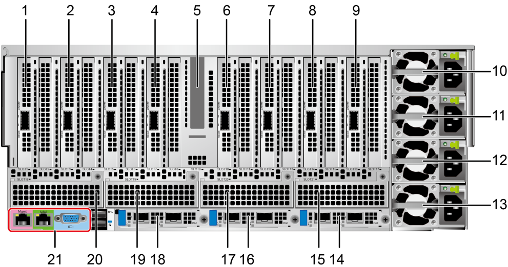
Figure 5-16 Rear view
