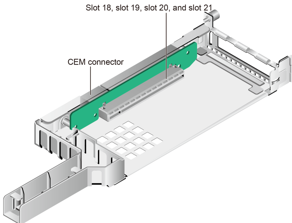
Figure 5-36 PCIe riser card
