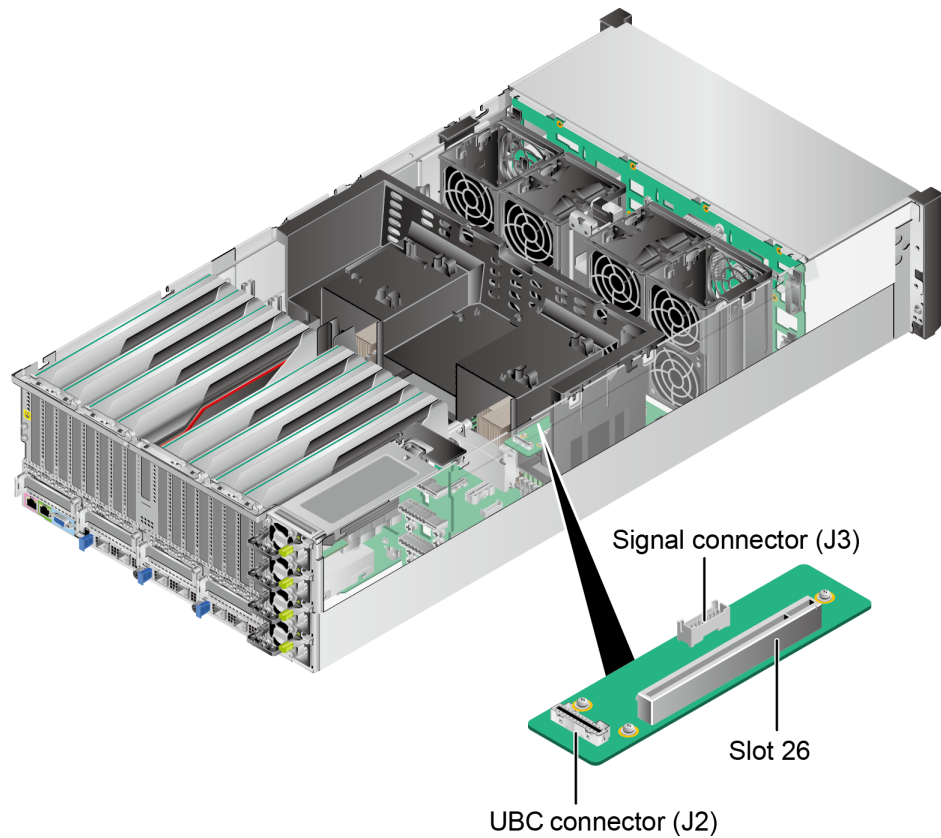
Figure 5-38 PCIe riser card (example: 24 x 3.5" Drive Configuration))
