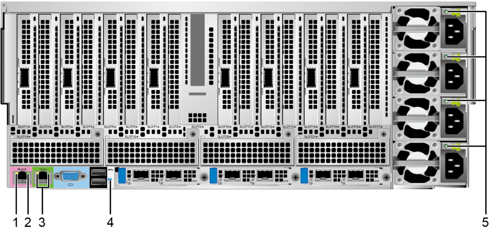
Figure 5-18 Indicators on the rear panel
