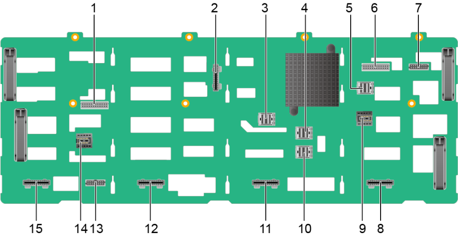
Figure 5-44 24 x 3.5" drive backplane (16 x SAS/SATA + 8 x NVMe/SAS/SATA)
