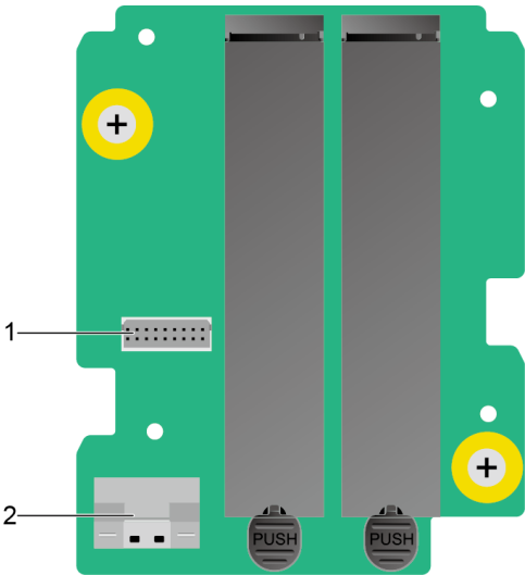
Figure 5-52 M.2 adapter board
