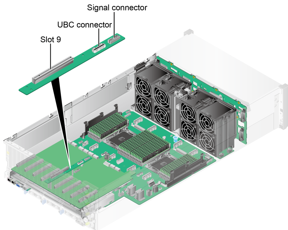
Figure 5-37 PCIe riser card
