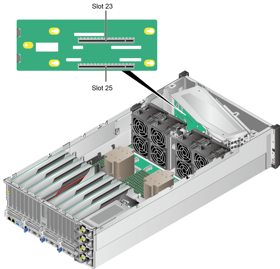
Figure 5-35 Front PCIe slots
