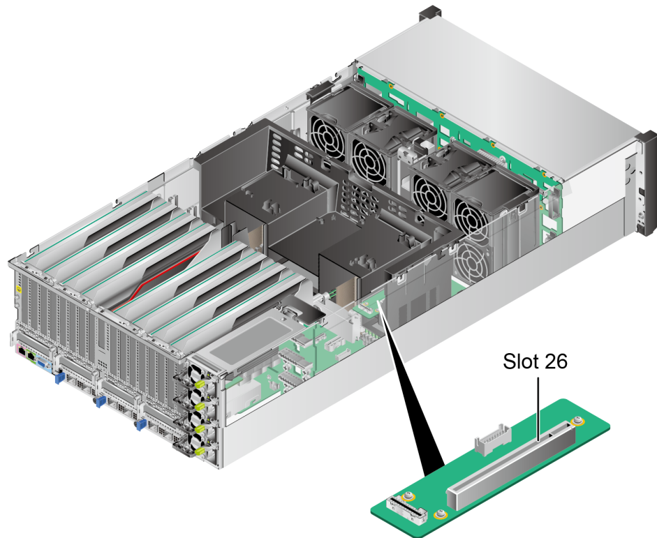
Figure 5-34 Built-in PCIe slot (example: 24 x 3.5" Drive Configuration))
