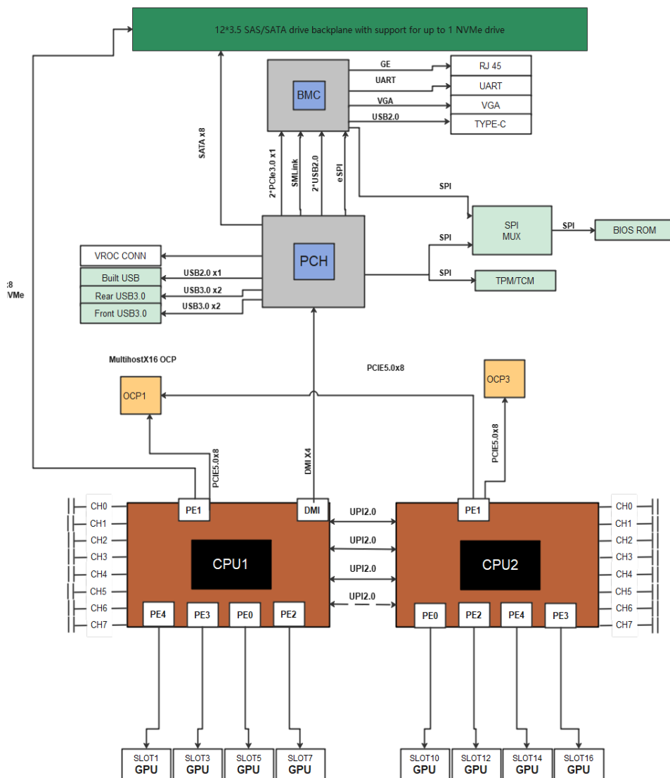
Figure 4-4 Logical structure 4 (configuration with 9 x 3.5" drives + 8 x dual-width GPU pass-through + 1 pass-through board)
