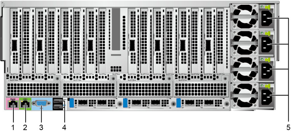
Figure 5-19 Ports on the rear panel
