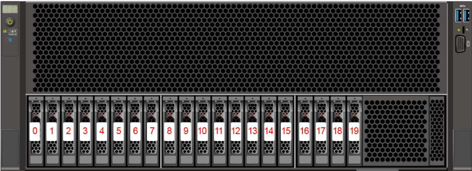
Figure 5-26 Drive numbering
