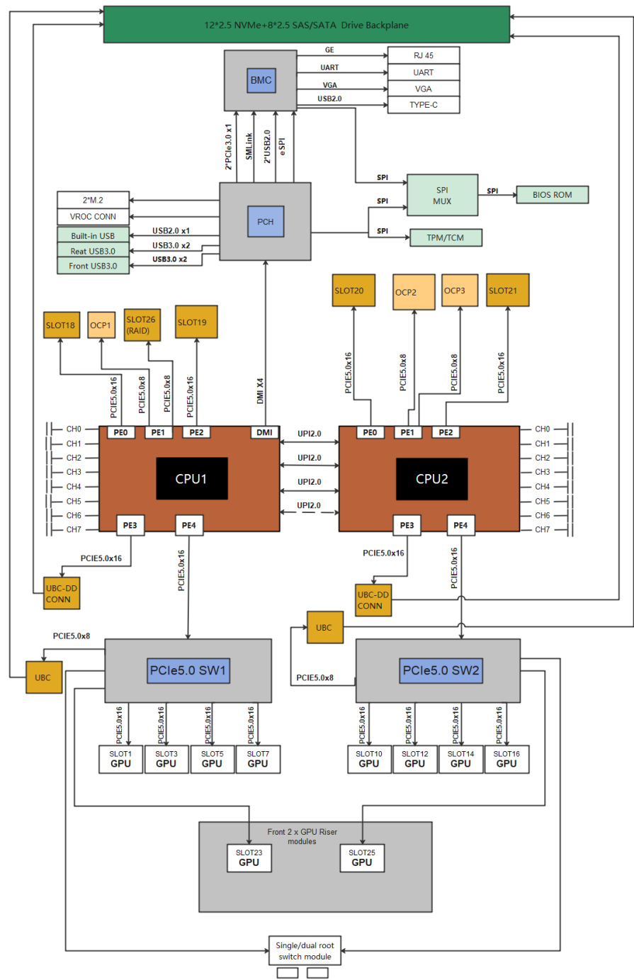
Figure 4-2 Logical structure 2 (configuration with 20 x 2.5" drives + 10 x dual-width GPUs + 1 x PCIe switch board)
