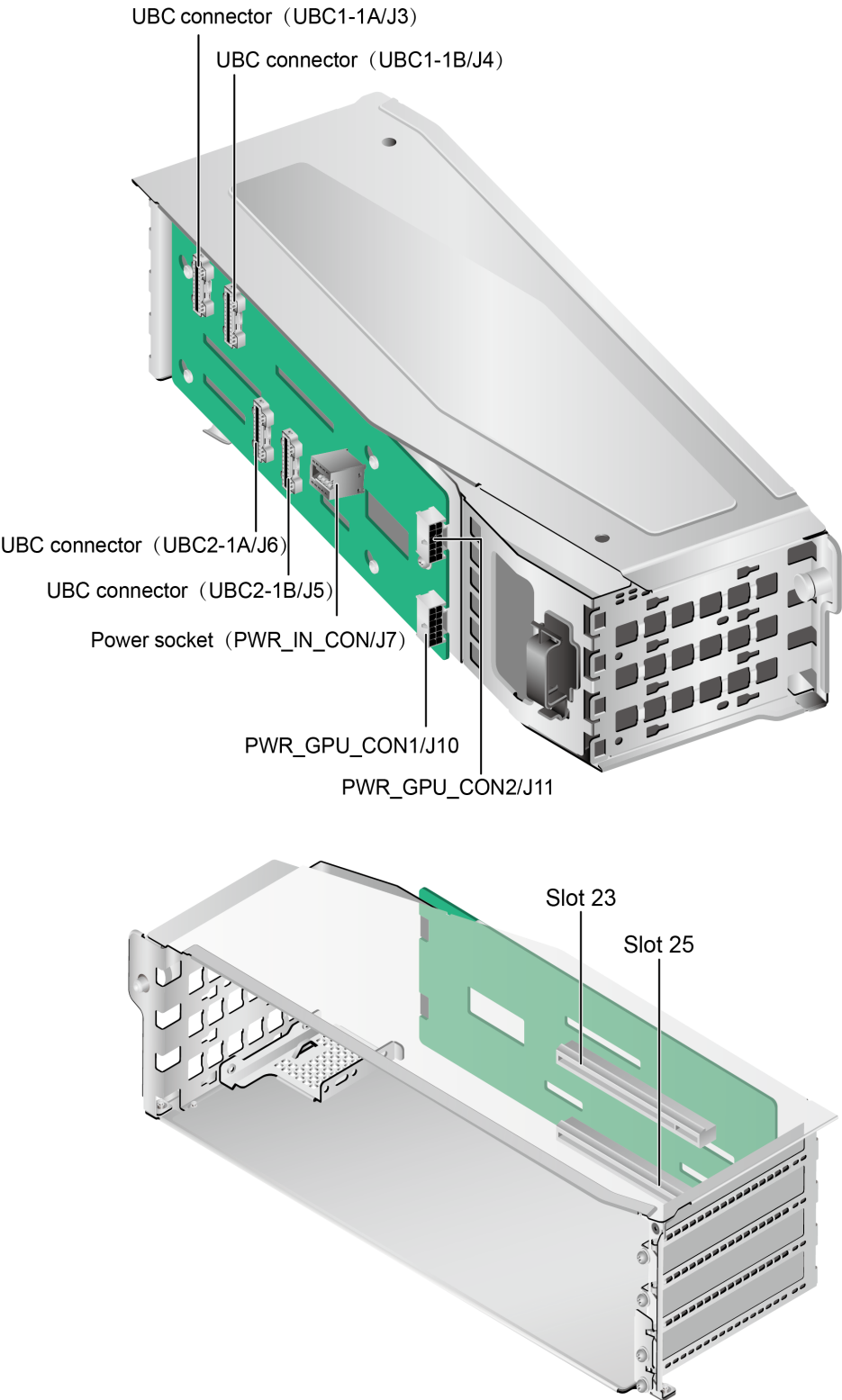
Figure 5-39 PCIe riser card
