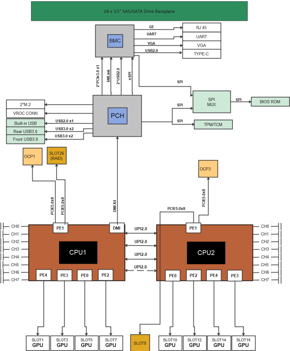
Figure 4-3 Logical structure 3 (configuration with 24 x 3.5" drives + 8 x dual-width GPUs pass-through board)
