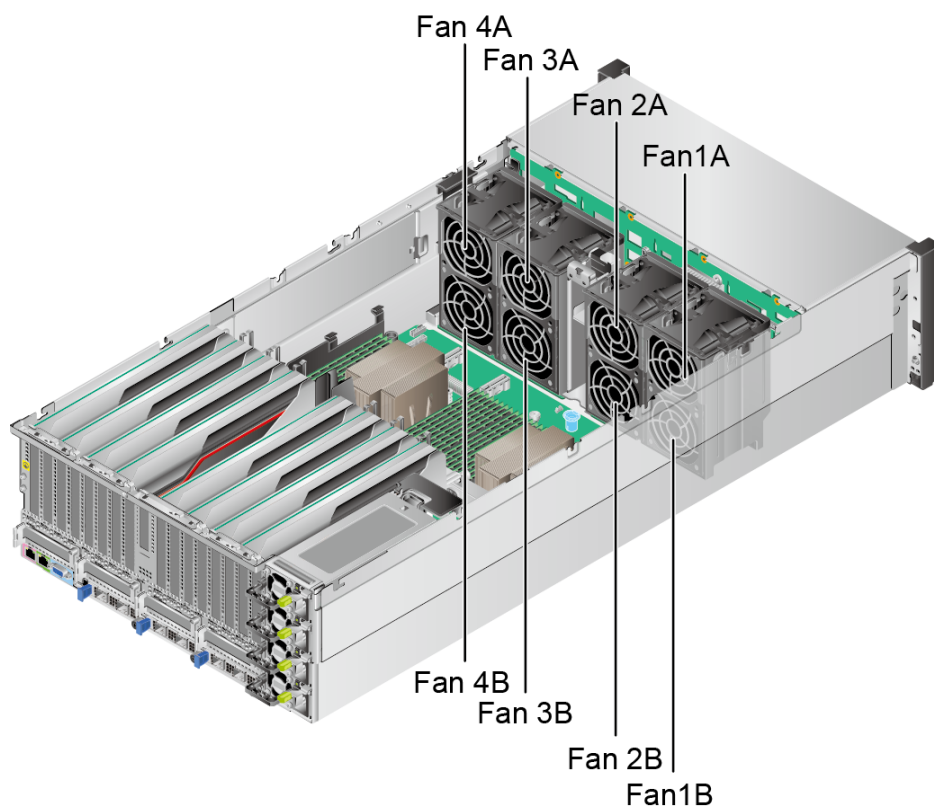
Figure 5-41 Positions of fan modules in a server with 20 x 2.5" drives (example)
