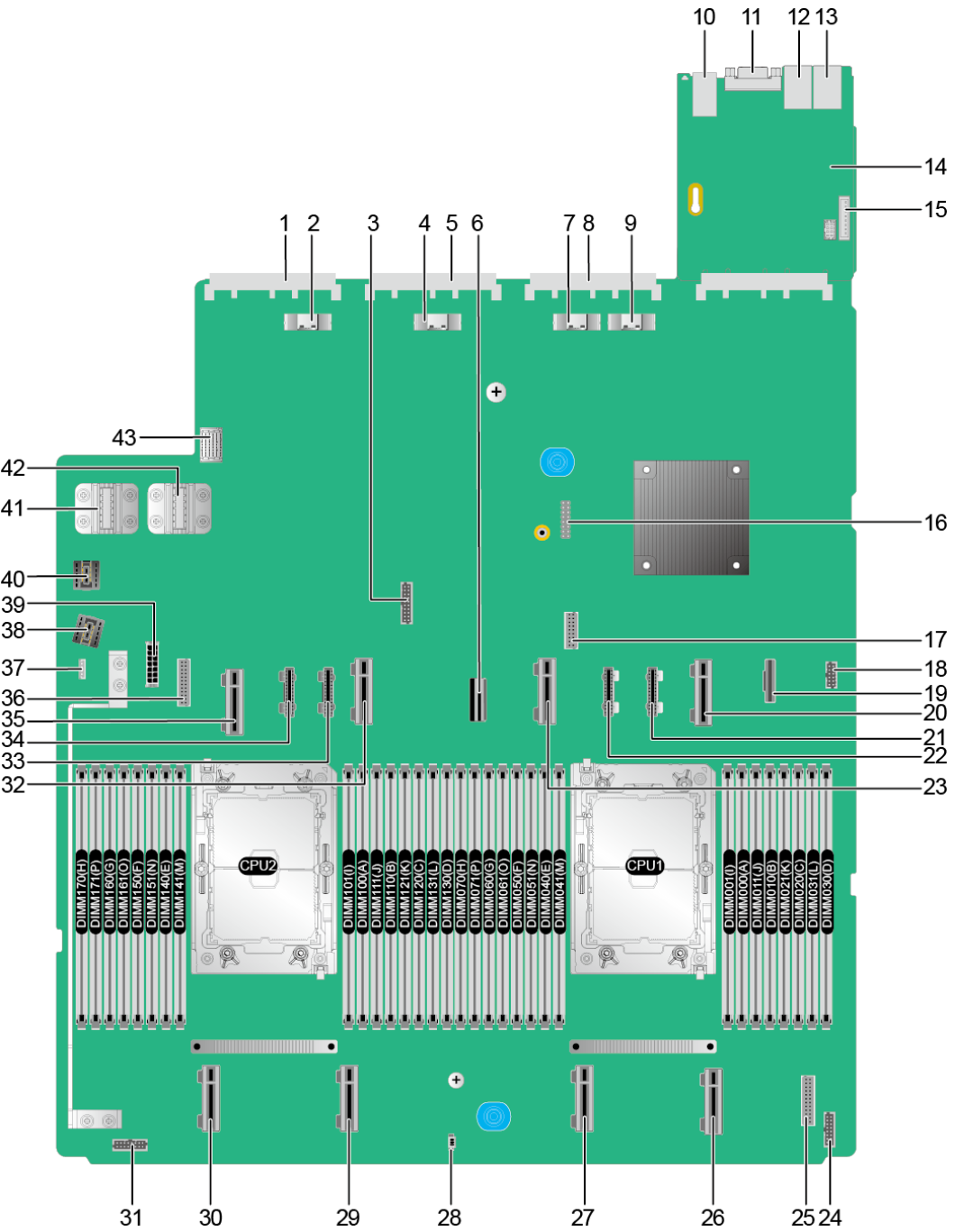
Figure 5-43 Mainboard (P/N code: 0302Y636)
