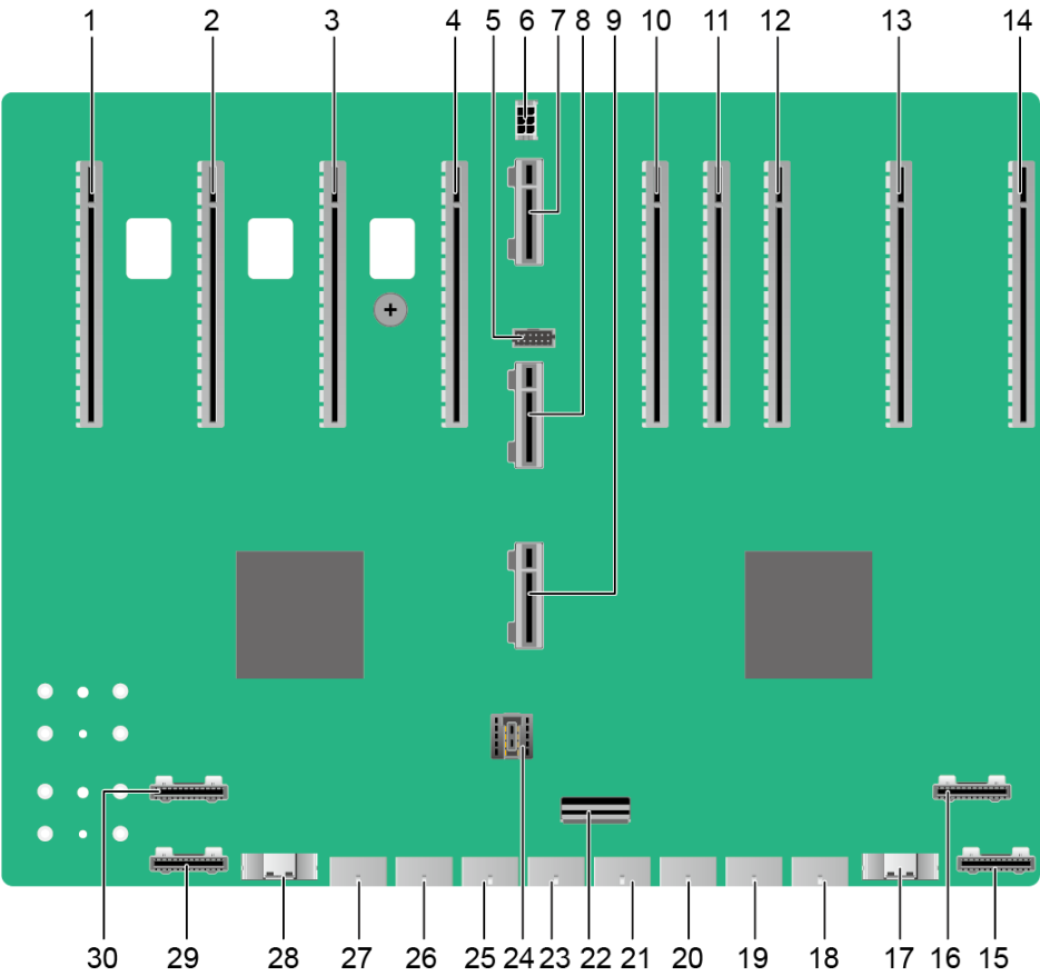
Figure 5-50 PCIe switch module 2
