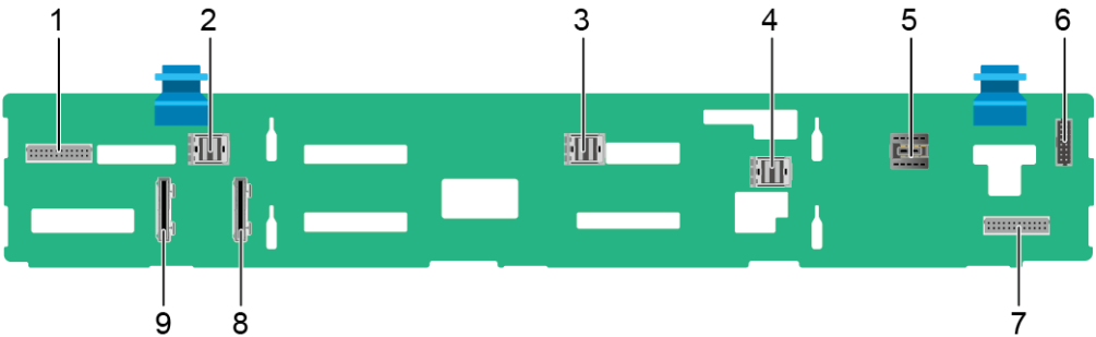
Figure 5-46 12 x 3.5" drive pass-through configuration backplane
