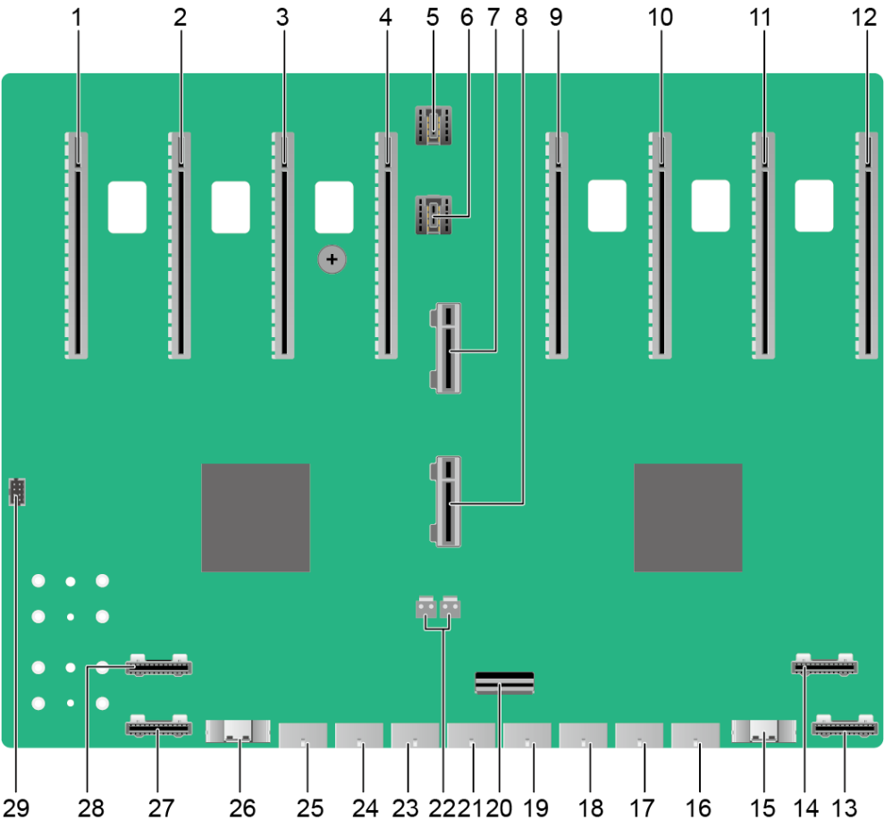
Figure 5-49 PCIe switch board 1
