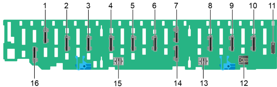
Figure 5-45 20 x 2.5" pass-through configuration backplane
