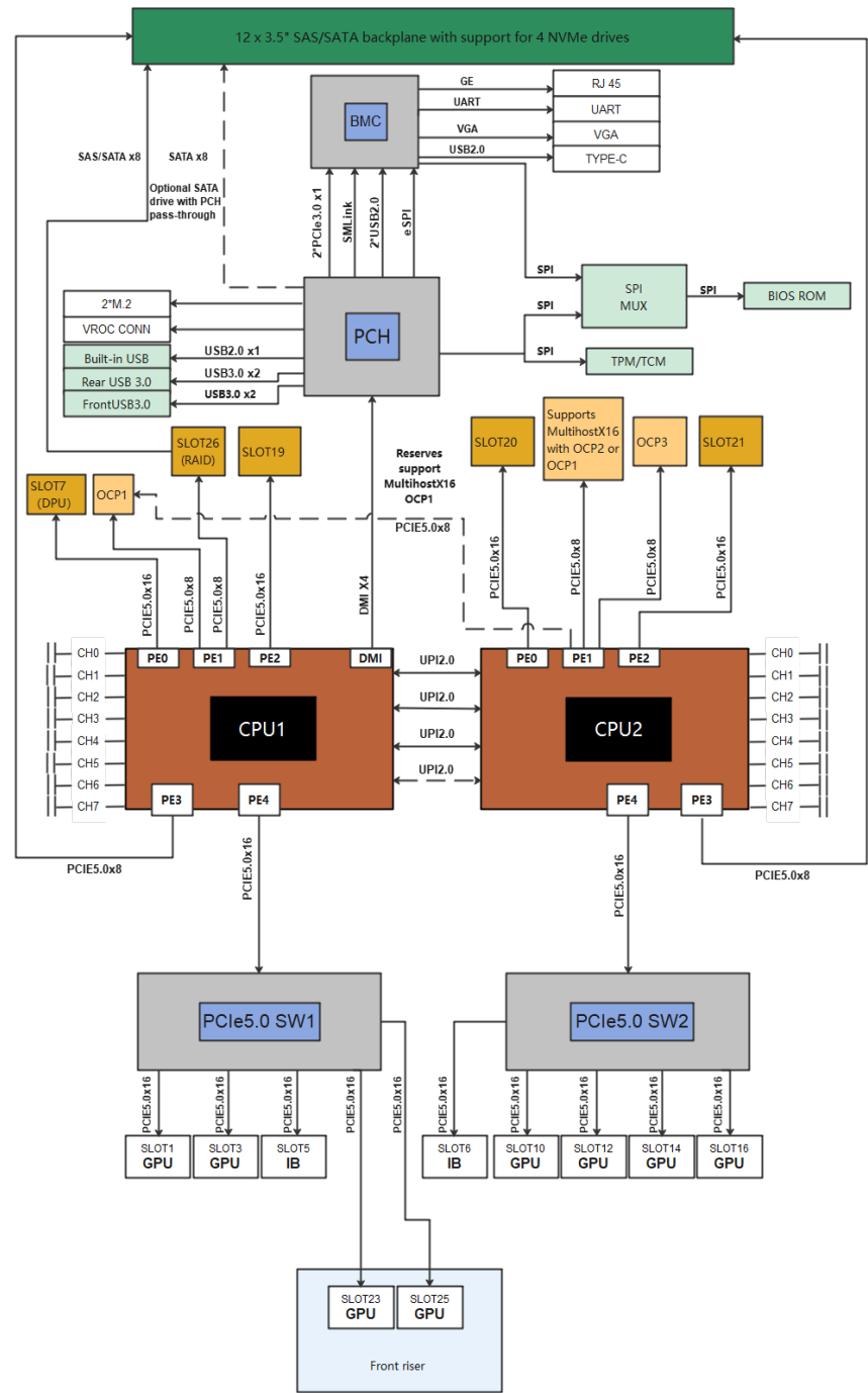
Figure 4-6 Logical structure 6 (configuration with 12 x 3.5" drives + 8 x dual-width GPUs + 1 DPU)
