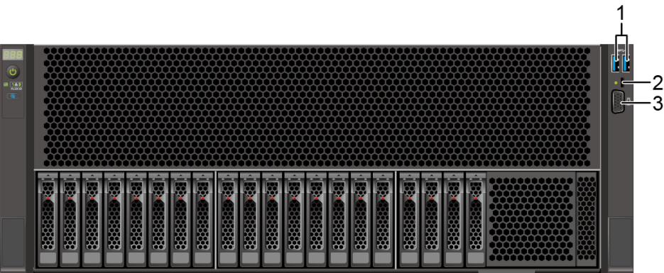
Figure 5-12 Ports on the front panel
