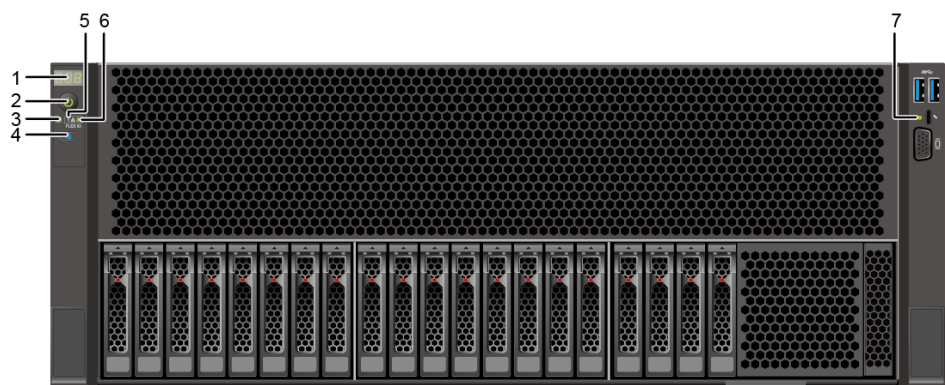
Figure 5-7 Indicators and buttons on the front panel
