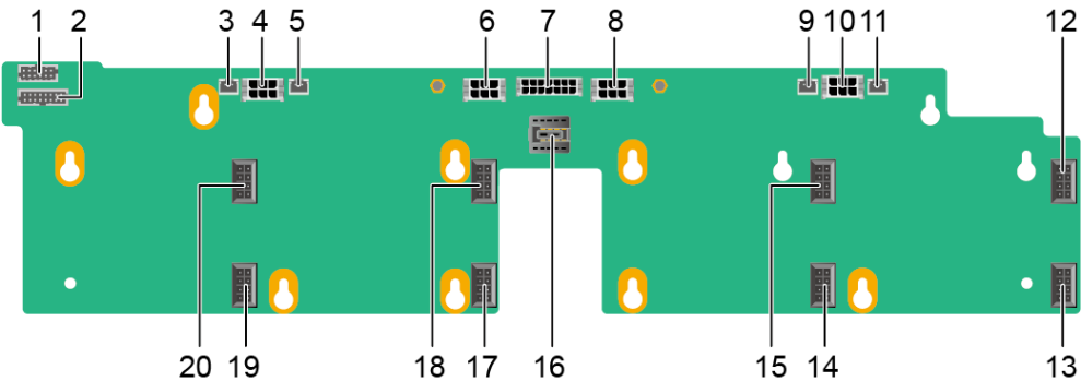
Figure 5-47 Fan board
