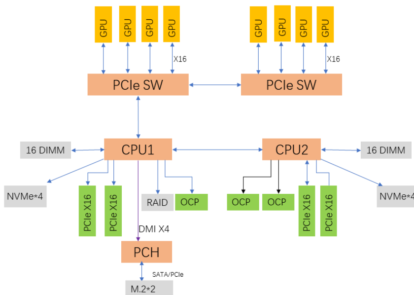
Figure 4-9 Cascaded topology
