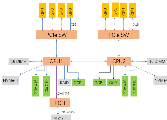
Figure 4-8 Balanced topology
