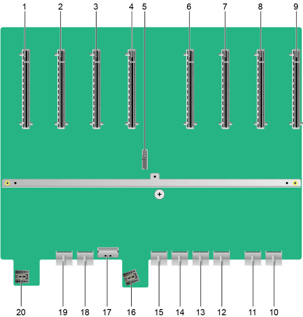
Figure 5-51 PCIe pass-through board
