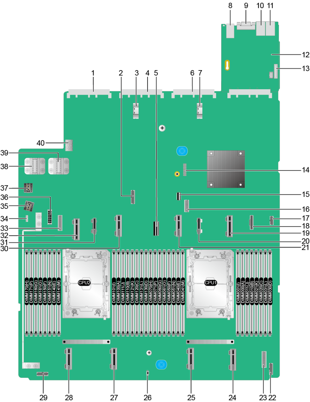
Figure 5-42 Mainboard (P/N code: 0302Y183)
