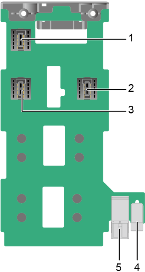
Figure 5-48 PSU backplane
