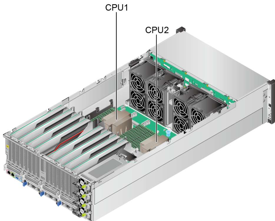
Figure 5-20 Positions of processors of a server with 24 x 3.5" drives (example)
