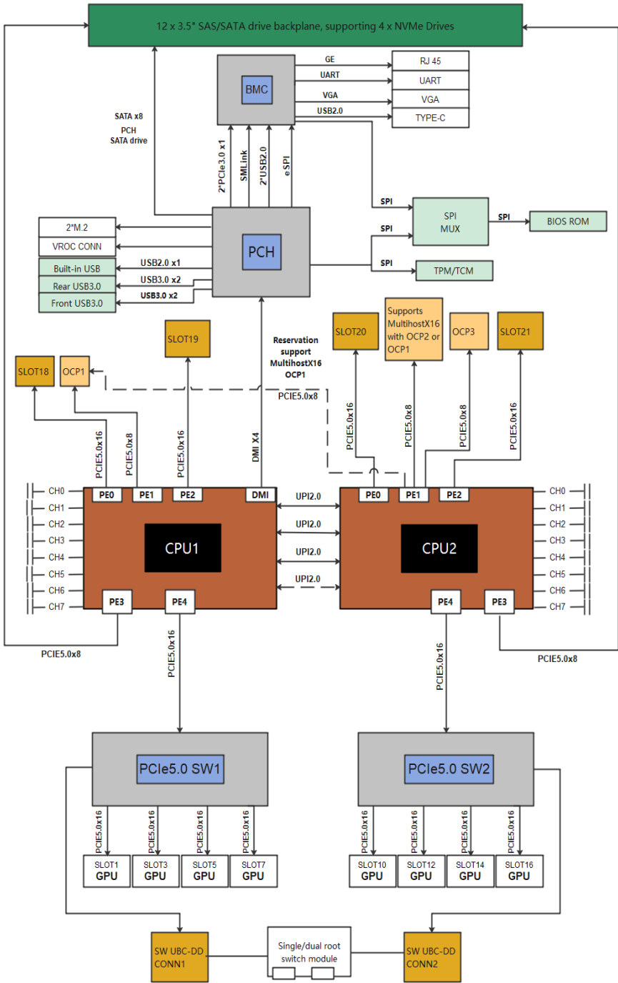
Figure 4-5 Logical structure 5 (configuration with 12 x 3.5" drives + 8 x dual-width GPUs + 1 x PCIe switch board)
