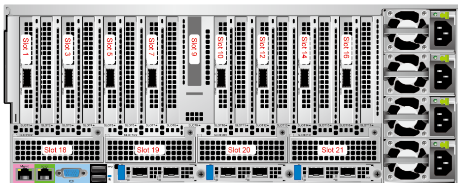
Figure 5-33 PCIe slots
