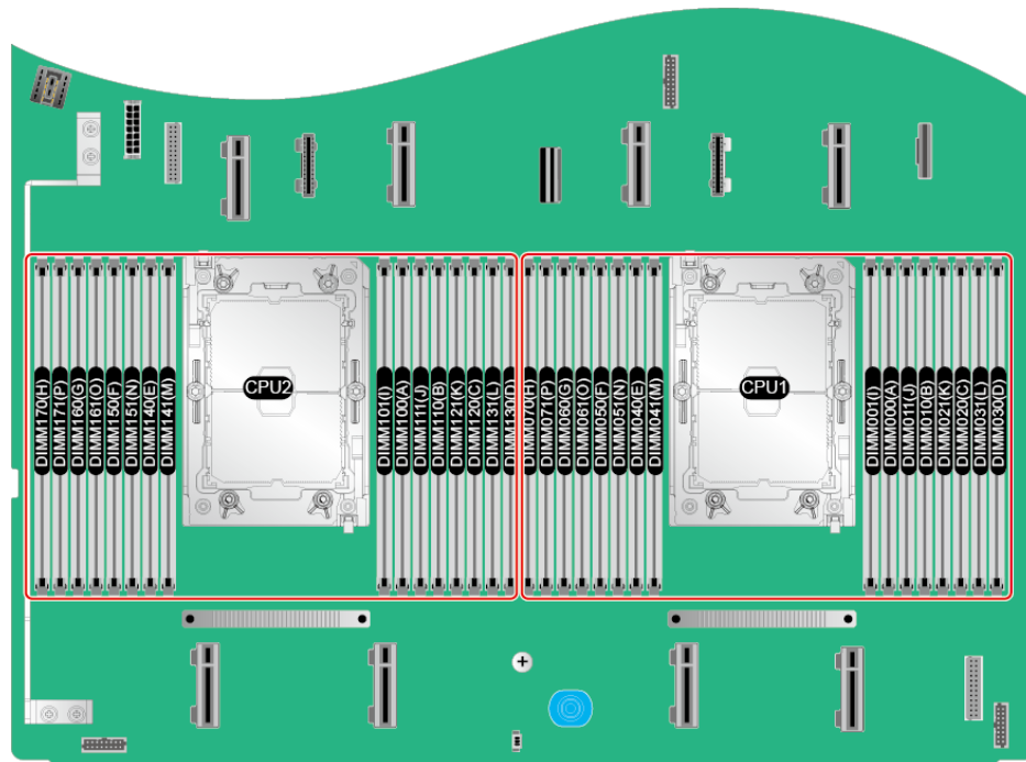
Figure 5-22 Positions of memory modules
